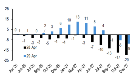
Figure 2: OIS forwards are now pricing in a roughly 50% probability of a hike in early 2027
